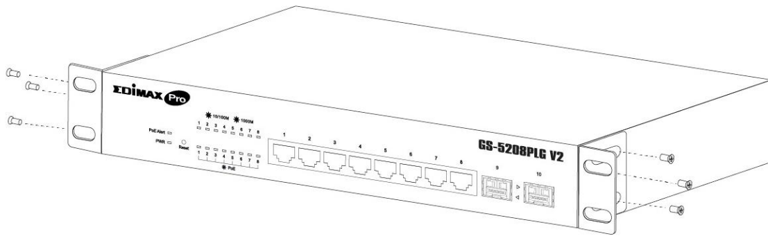
Figure 5 – Bracket Installation
